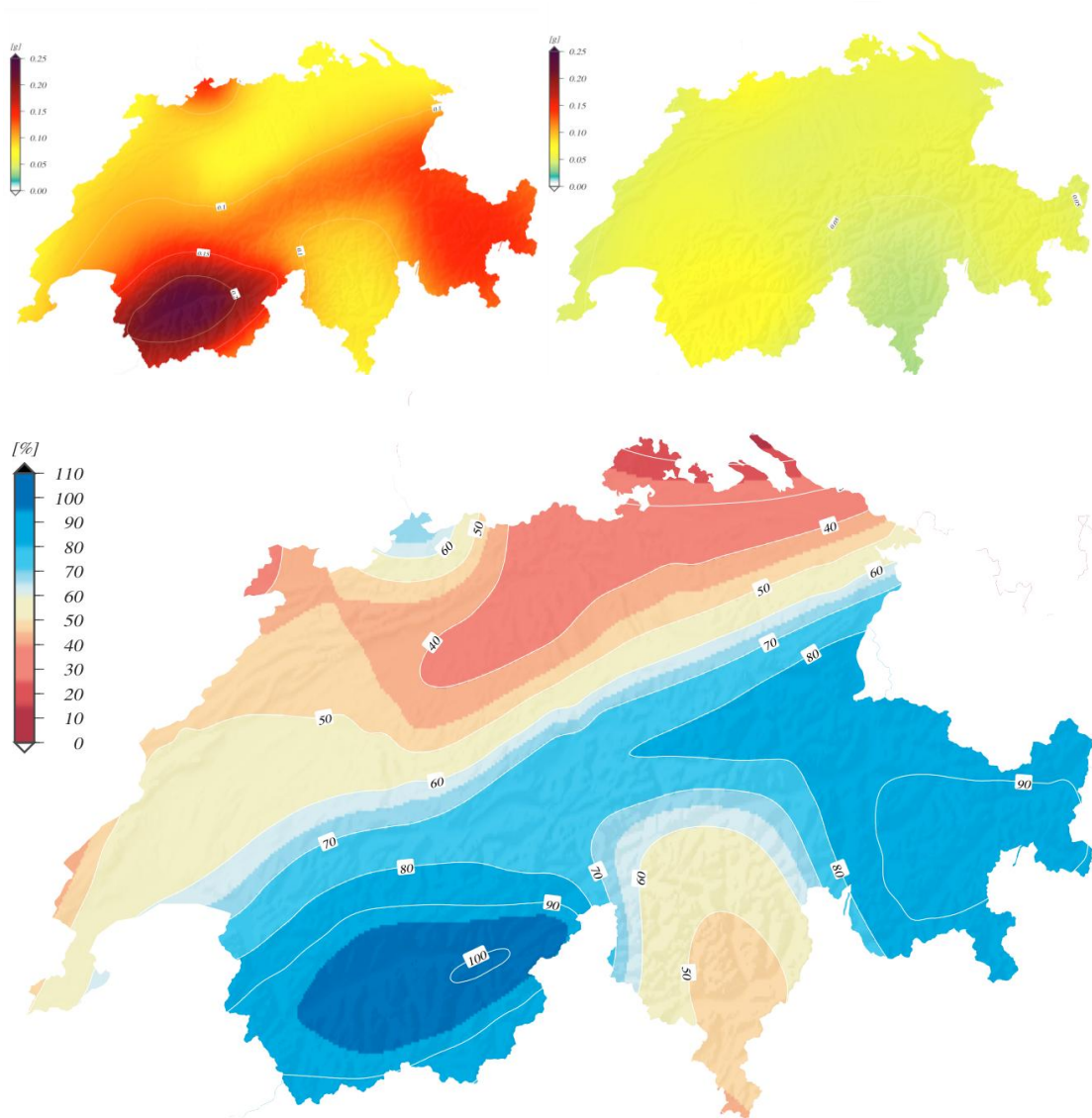
Figure 77: Percentage difference of the two-ground motion hazard map in terms of SA[0.2s] for mean return maps of 475 yrs as obtained for the shallow (top left) and the deep sources (top right) and their corresponding ground motion logic tree branches.
