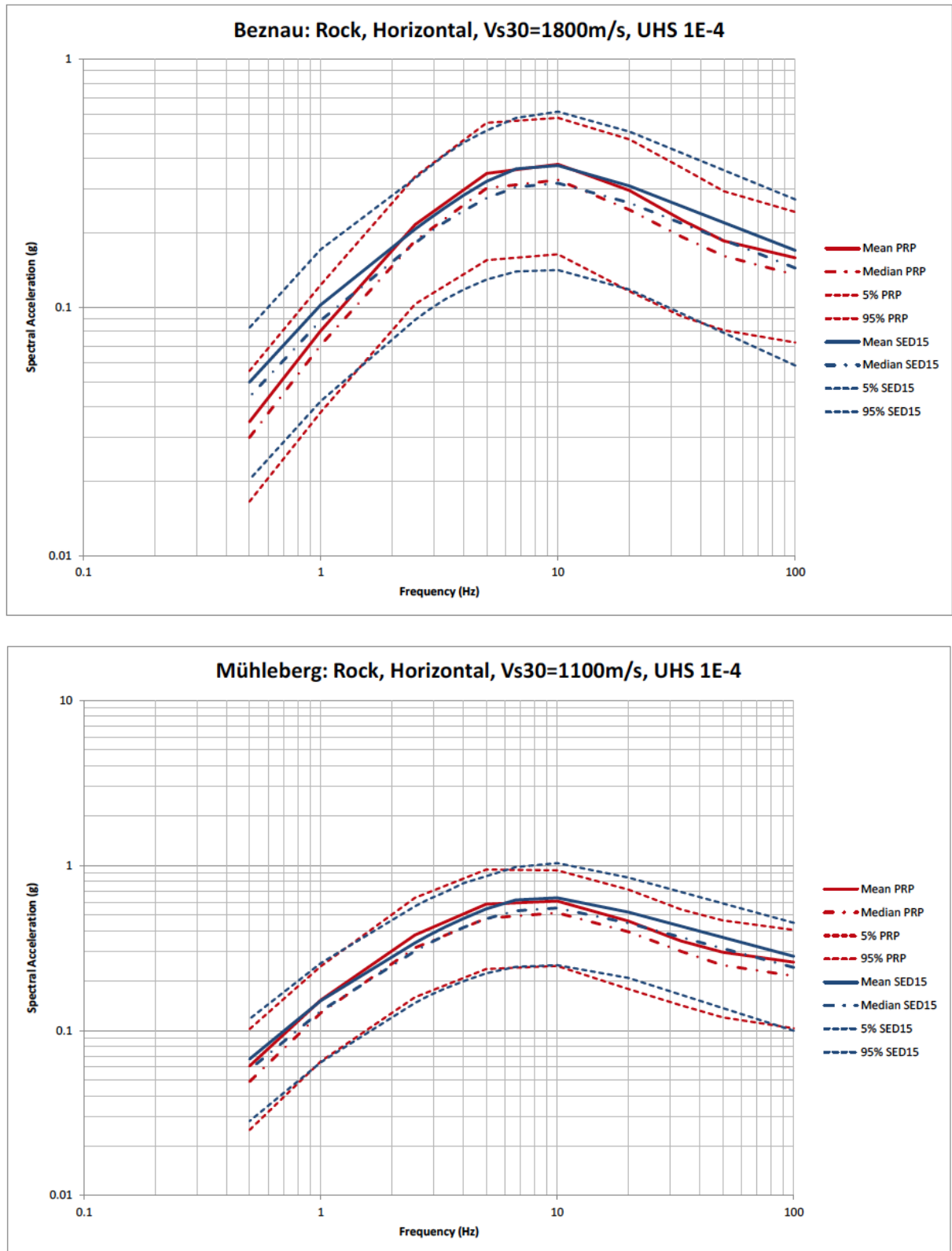
Figure 85: Rock hazard comparison for the site Beznau at an annual probability of exceedance of 1E-4 for PRP and SED 2015.
