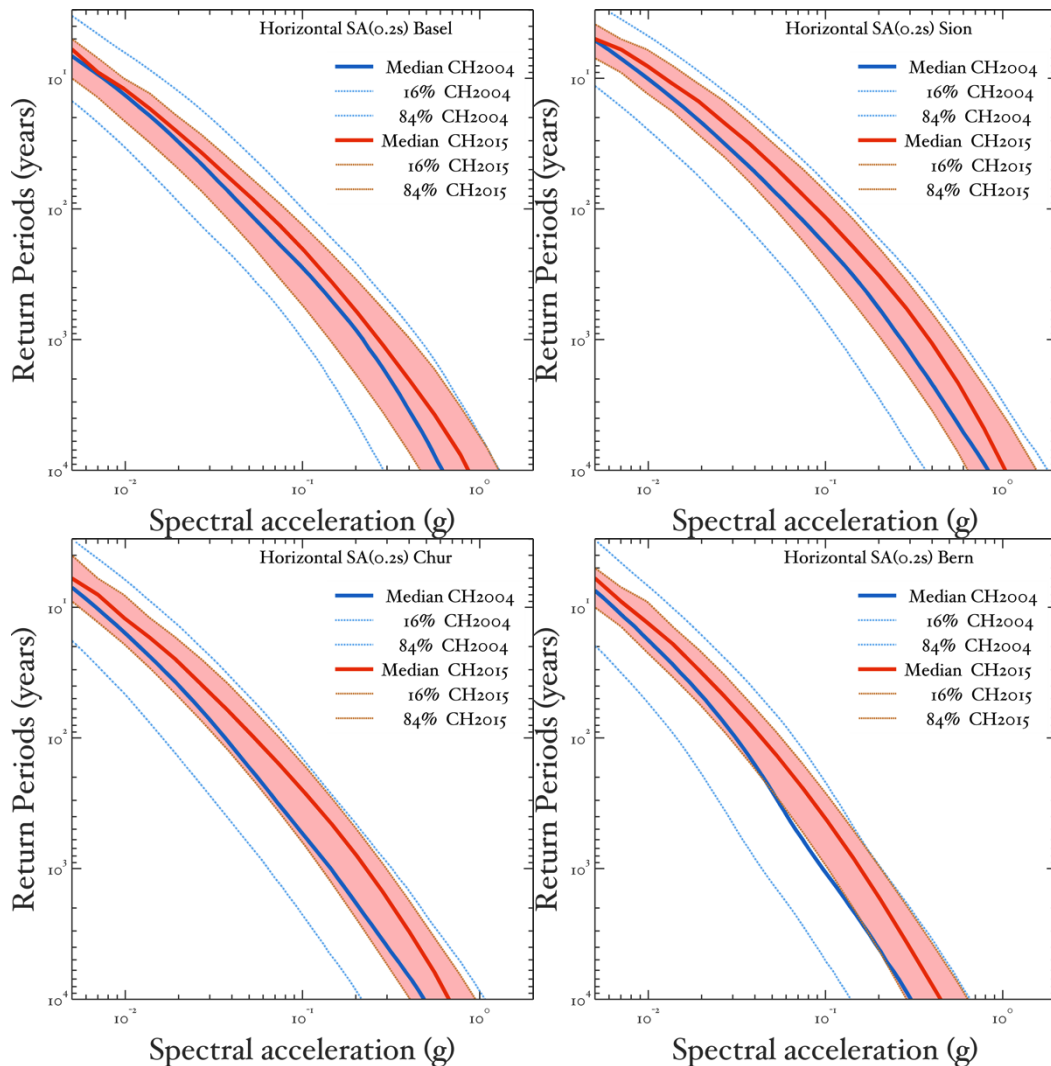
Figure 72: Hazard curves in terms of S_a[0.2s] of the 2015 and 2004 ground motion hazard for the cities of Basle, Sion, Chur and Bern. The median (50 th ) values are shown with continuous lines for 2015 (red) and 2004 (blue). The uncertainty range is illustrated with dashed lines of similar colours.
