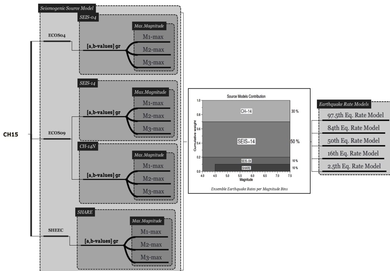
Figure 34: Schematic illustration of the seismogenic source logic tree.
