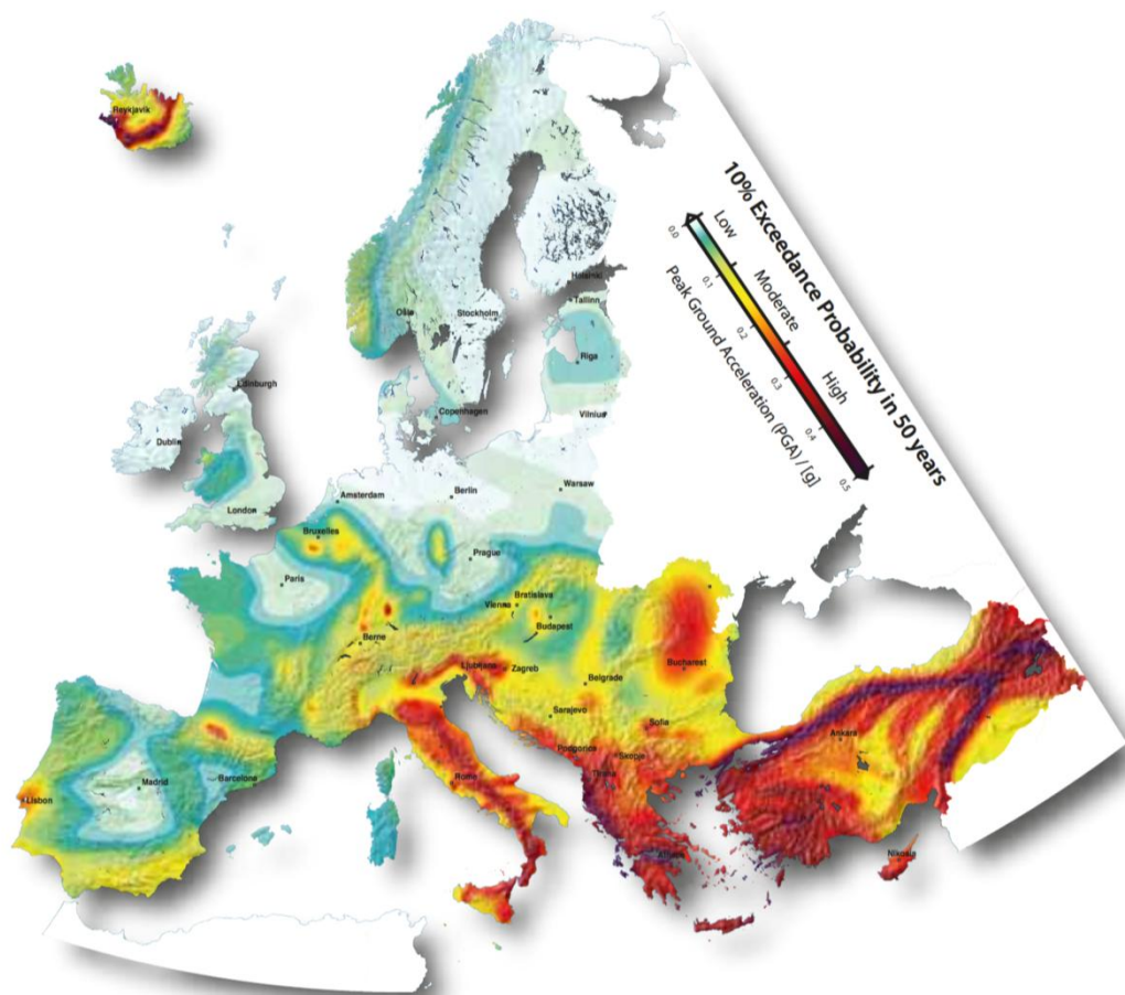
Figure 4: The SHARE European Seismic Hazard Map displays the ground motion (i.e. the Peak Ground Acceleration PGA) expected to be reached or exceeded with a 10% probability in 50 years, i.e. these values repeat themselves on average every 475 years. Cold colours indicate comparatively low hazard areas ( \text{PGA} \leq 0.1\text{g} ), yellow to orange colours indicate moderate hazard areas ( 0.1 < \text{PGA} \leq 0.25\text{g} ) and red colours indicate high hazard areas ( \text{PGA} > 0.25\text{g} ).
