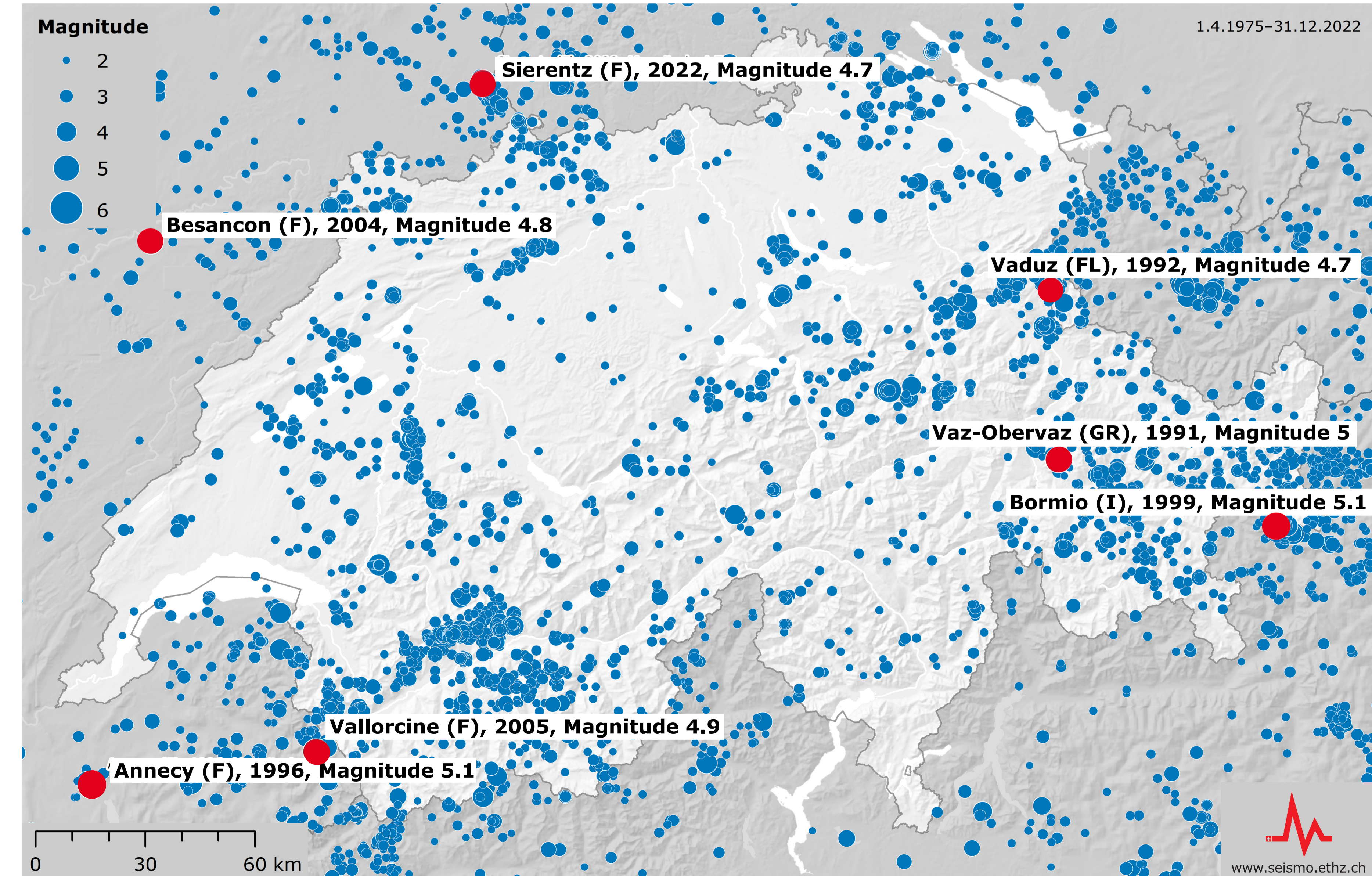
The strongest earthquakes since 1975
