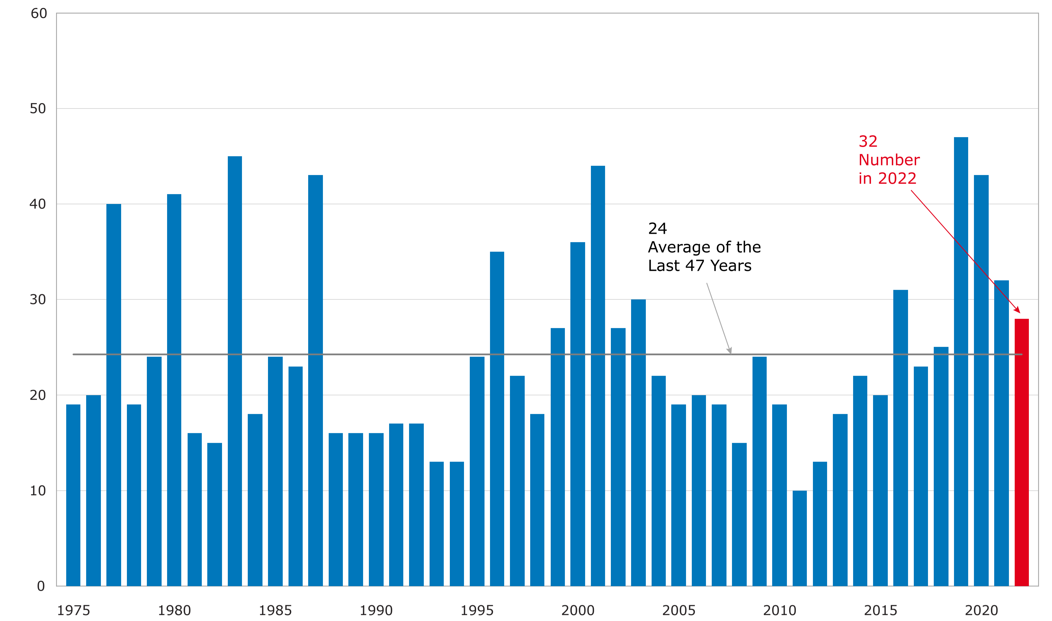
Number of Earthquakes with Magnitude 2.5 or Greater per Year
